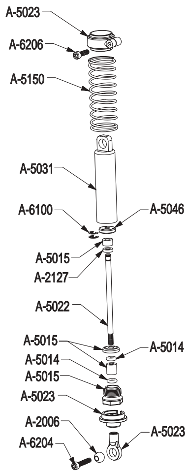
REAR SHOCK
